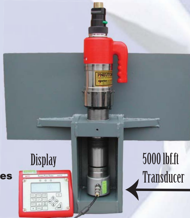
Stand-Alone Test System
